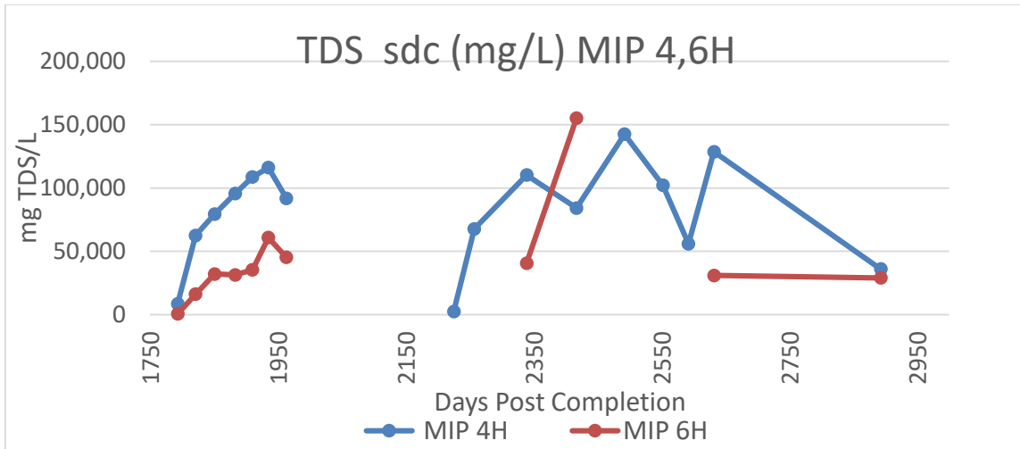
Figure 4.3. Changes in produced water TDS sdc (sum of dissolved constituents) through the first 1793 through 2893 days post completion (4,6H).
