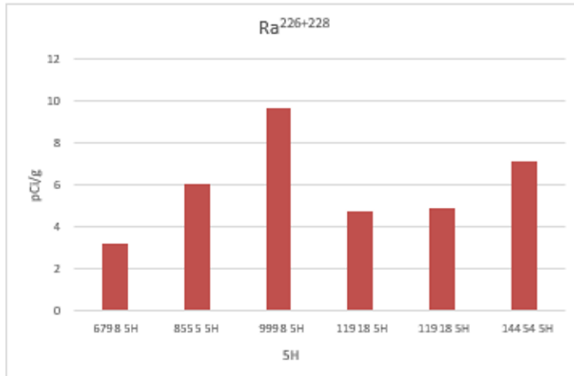
Figure 4.15. Combined Ra 226 + 228 for 5H MIP sites.
