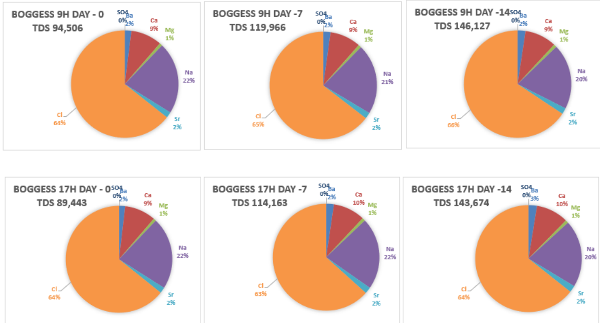
Figure 4.17. Major ion concentrations in produced water from wells BOGCESS 9H and 17H.
