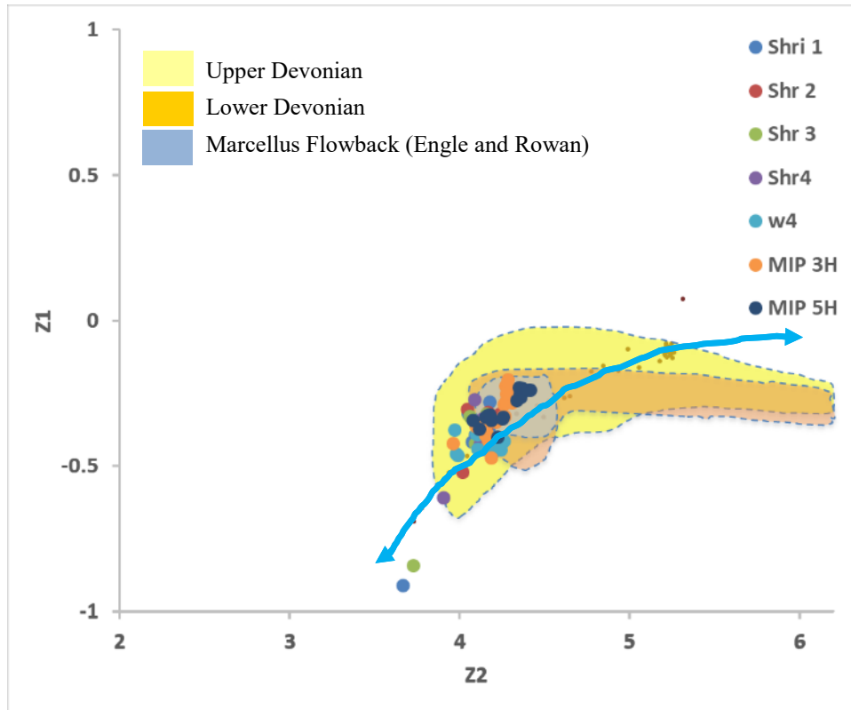
Figure 3.1 irl plot (Na-Cl-Br) redrafted after Engle and Rowan (2014) with flowback fluids from both the MSEEL site (MIP 3H and 5H) and the UPP wells (Shr 1-4 and W4). The blue line represents modern seawater evaporation pathway. The data plot along a trajectory that is consistent with evaporated paleo seawater.
