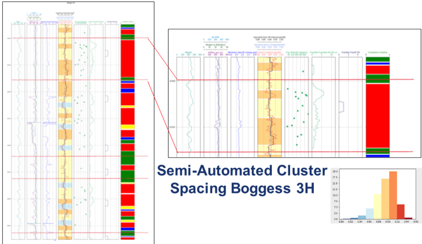
Figure 1.6: Display of a single stage of Boggess 3H showing Sh_{min} derived from accelerometer data in track 4 and color coded and grouped by Sh_{min} bin. Track 6 shows the number of fractures per foot from the LWD image logs. The rightmost track is a risk grading from high risk (red) to low risk (green). The five clusters were adjusted to target the green areas with a consistent Sh_{min} and avoid fractures.
