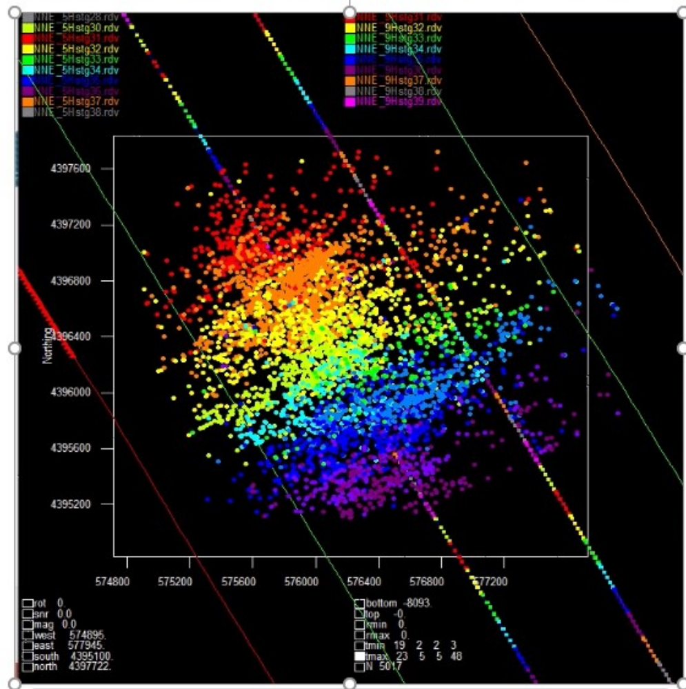
Figure 1.4: Microseismic events for eight stages of the Boggess 5H well showing the large number of events recorded using the permanent fiber in the 5H and the deployable fiber in in the 1H. Colors are by stages.
