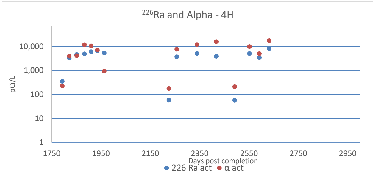
Figure 4.9. The relationship between gross alpha and 226 Ra as a function of time post completion at 4H.
