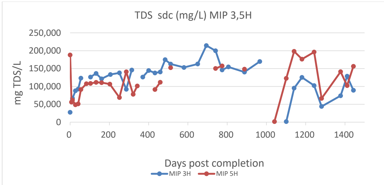
Figure 4.2. Changes in produced water TDS sdc (sum of dissolved constituents) through the first 1443 days post completion (3,5H).
