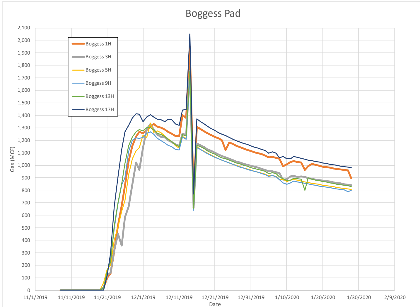
Figure 1.3: Initial daily net production from the Boguess Pad adjusted for Mcf per 1000' of completed lateral. The wells engineered using the MSEEL software are highlighted with thicker lines (1H and 3H). As you can see outside wells (1H and 17H) perform better than interior wells due to reduced competition. Also wells engineered using the MSEEL approach got off to a slower start but have narrowed the gap in daily production and in the case of the 3H, it is producing more than any other interior well. In the case of the 17H more sand was used per stage and we need to adjust for sand per foot. The production is very early and the picture could very easily change.
