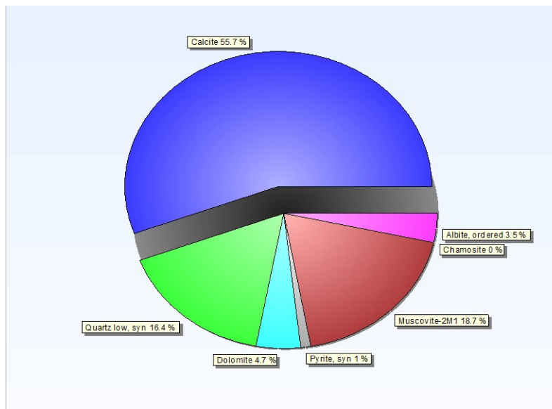
Figure 3.3c UPP Rietveld quantification of target formation as a pie chart, showing mineral composition in weight percent.
