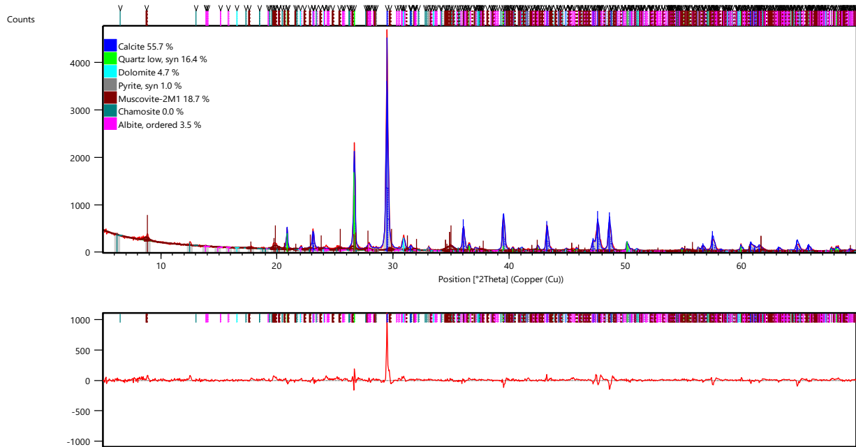
Figure 3.3b UPP Rietveld quantification of target formation, showing mineral composition in weight percent, and the difference plot derived from the whole pattern fitting.
