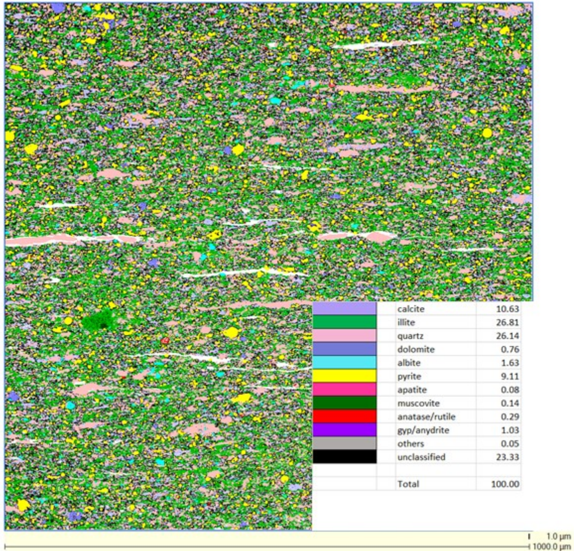
Figure 3.4a MSEEL QEMSCAN mineral map of ~1 mm 2 region of Lower Marcellus (depth 7543.0'). Compared to the Point Pleasant, this hydraulic fracturing target is very different in mineral composition and texture. The same general color scheme for minerals is used as in Figure UPP QEMSCAN. Green shades are illitic clay (25.7 %); light pink is quartz (25.2 %); black unclassified mixed pixels (22.5 %); light lavender is calcite (10.3 %); yellow is pyrite (8.8 %); cyan is albite (1.6 %); white is large OM macerals (3.4 %); purple is gypsum/anhydrite (1 %); dark lavender is dolomite (0.7 %). Remaining < 1% includes small quantities of mica as biotite, muscovite and glauconite, titania, Ca-phosphate, and K-feldspar. The black unclassified pixels represent the complex clay fraction, with the finest-grained OM intercalated with illitic clay, barite, pyrite, REE phosphates, sphalerite (ZnS) and a U-Ti phase, as identified by EDX spot analysis. This Lower Marcellus is a very OM-rich siliciclastic mudrock with minor carbonate; much of the large OM macerals are replaced by quartz to varying degrees.
