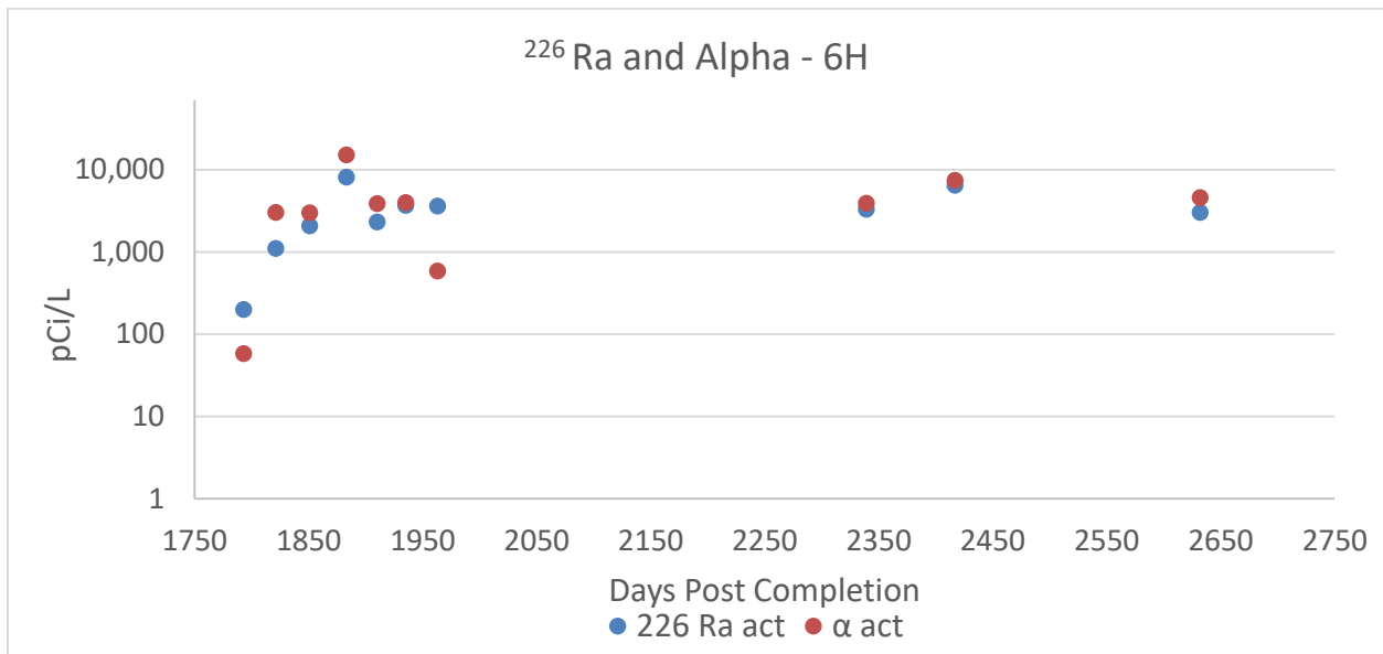
Figure 4.10. The relationship between gross alpha and 226 Ra as a function of time post completion at 6H.
