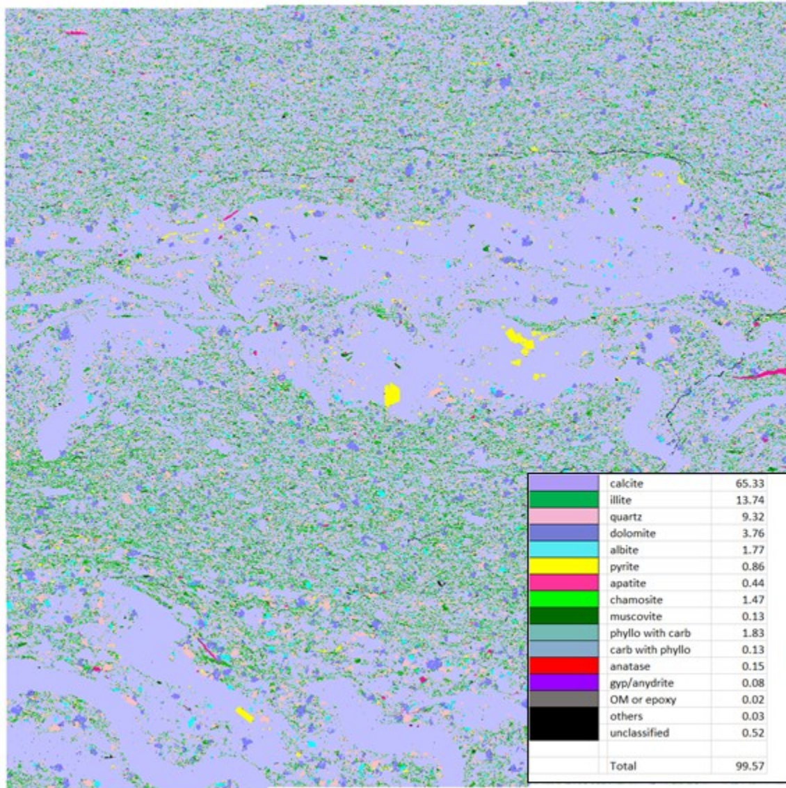
Figure 3.3a UPP QEMSCAN. QEMSCAN mineral map of ~3x3 mm 2 region of polished thin section of Point Pleasant hydraulic fracturing target (depth ~8550'). Lavender shades are calcite and dolomite (dark lavender), green shades are mainly illitic clay (with minor muscovite and chamosite), light pink is quartz, cyan is albite, yellow is pyrite, and fuchsia is apatite. Organic matter (OM, arrowed) is black; much of it is finely intercalated with illitic clay and too small to be resolved with QEMSCAN. Desiccation cracks also are black in this image.
