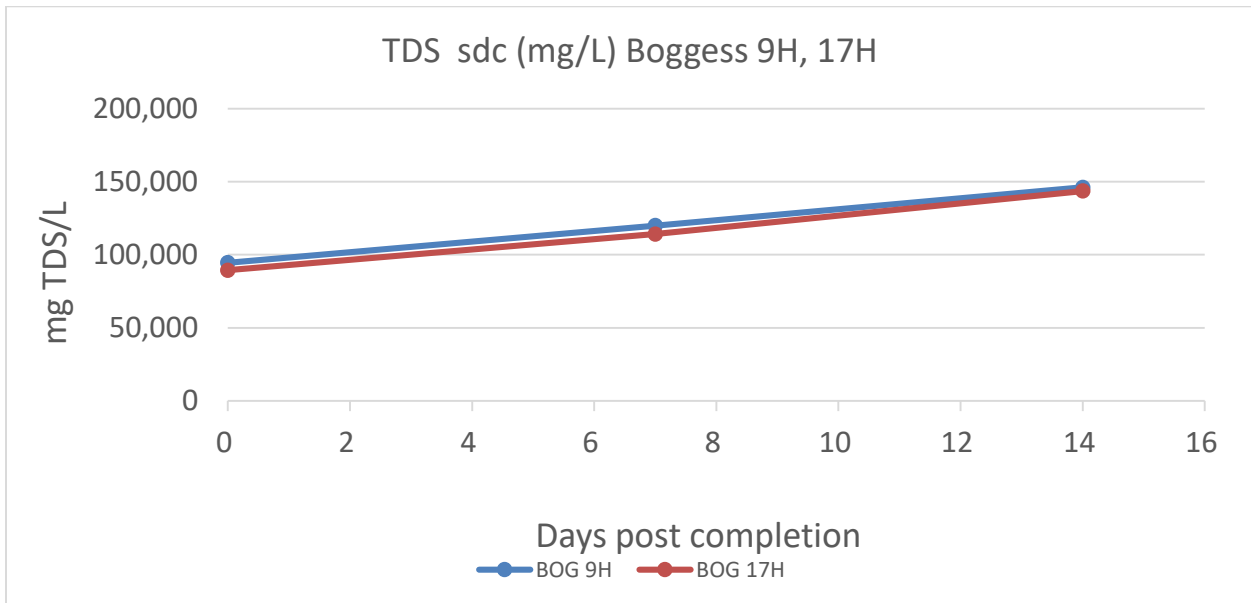
Figure 4.18. TDS (sd) at Boggess 9H and 17H; days 0-14.
