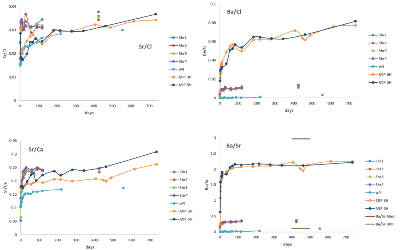
Figure 3.2 Elemental ratios for UPP and MSEEL fluids (wt:wt ratios). Top left Sr/Cl, bottom left Sr/Ca, top right Ba/Cl and bottom right Ba/Sr in flowback fluids from MSEEL and UPP wells showing an increase in the Ba/Cl and Sr/Cl ratios over time. The increase in alkaline earth elements compared to Cl reflects ion exchange reactions and dissolution of Sr and Ba bearing phases such as barite/celestite or gypsum, carbonates, or phosphate minerals.
