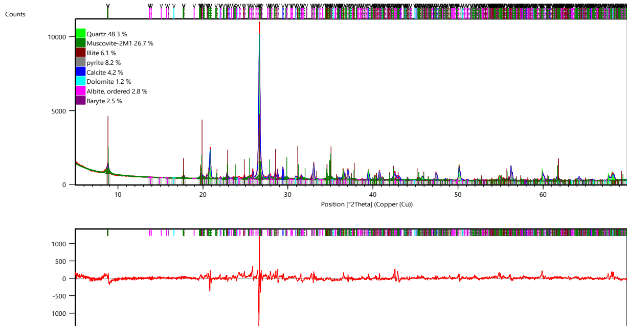
Figure 3.4b MSEEL Rietveld quantification of target formation, showing mineral composition in weight percent, and the difference plot derived from the whole pattern fitting.
